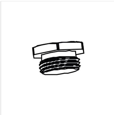
7 Oxygen Sensor Port Plug, M18 x 1.5
